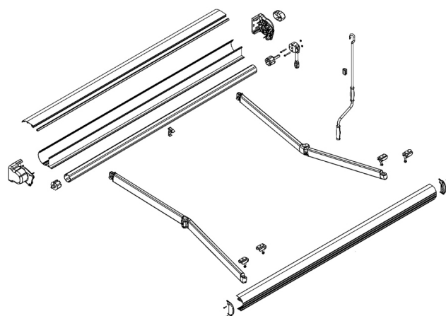
Base Plus despiece
