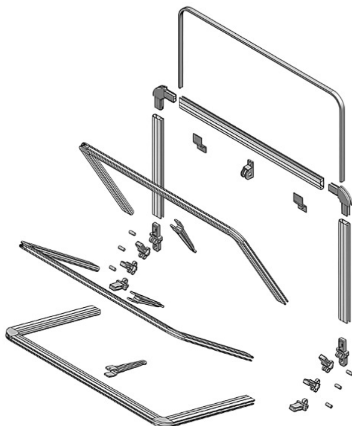
Capota despiece
