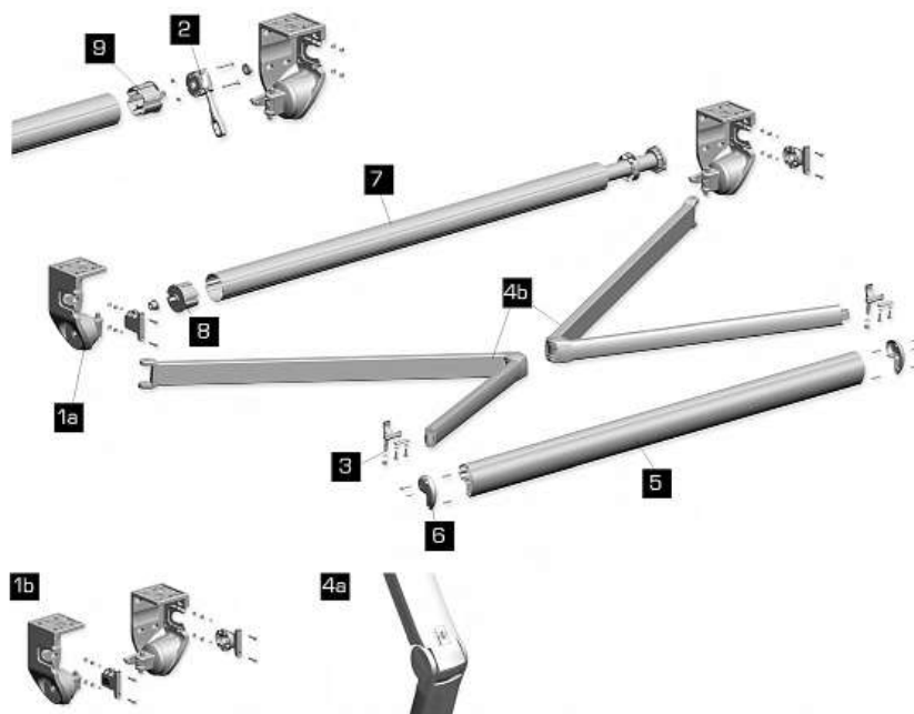
Marboré despiece
