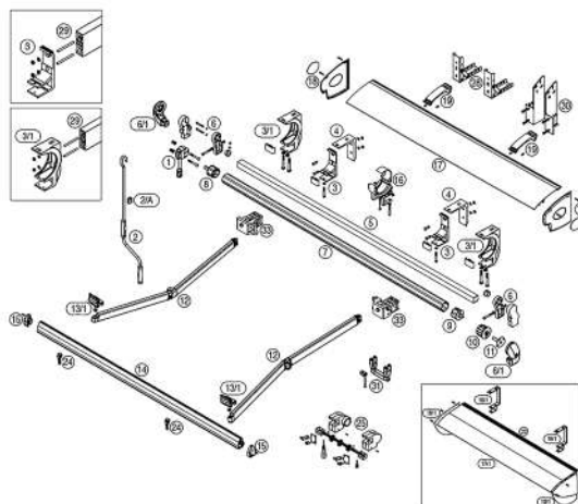
Monoblock 2.0 despiece
