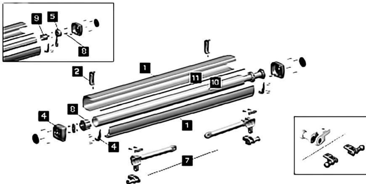
Vertical estor Microbox despiece
