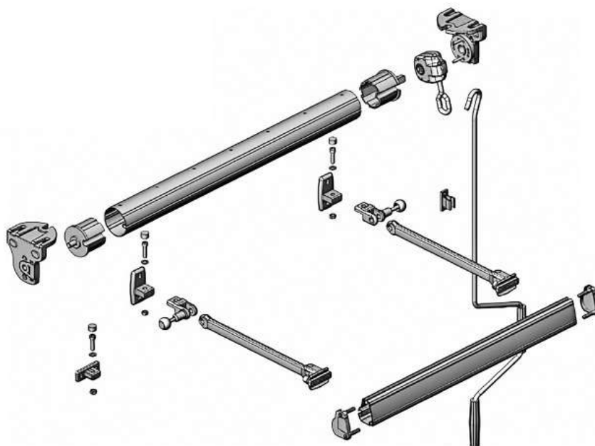
Vertical despiece
